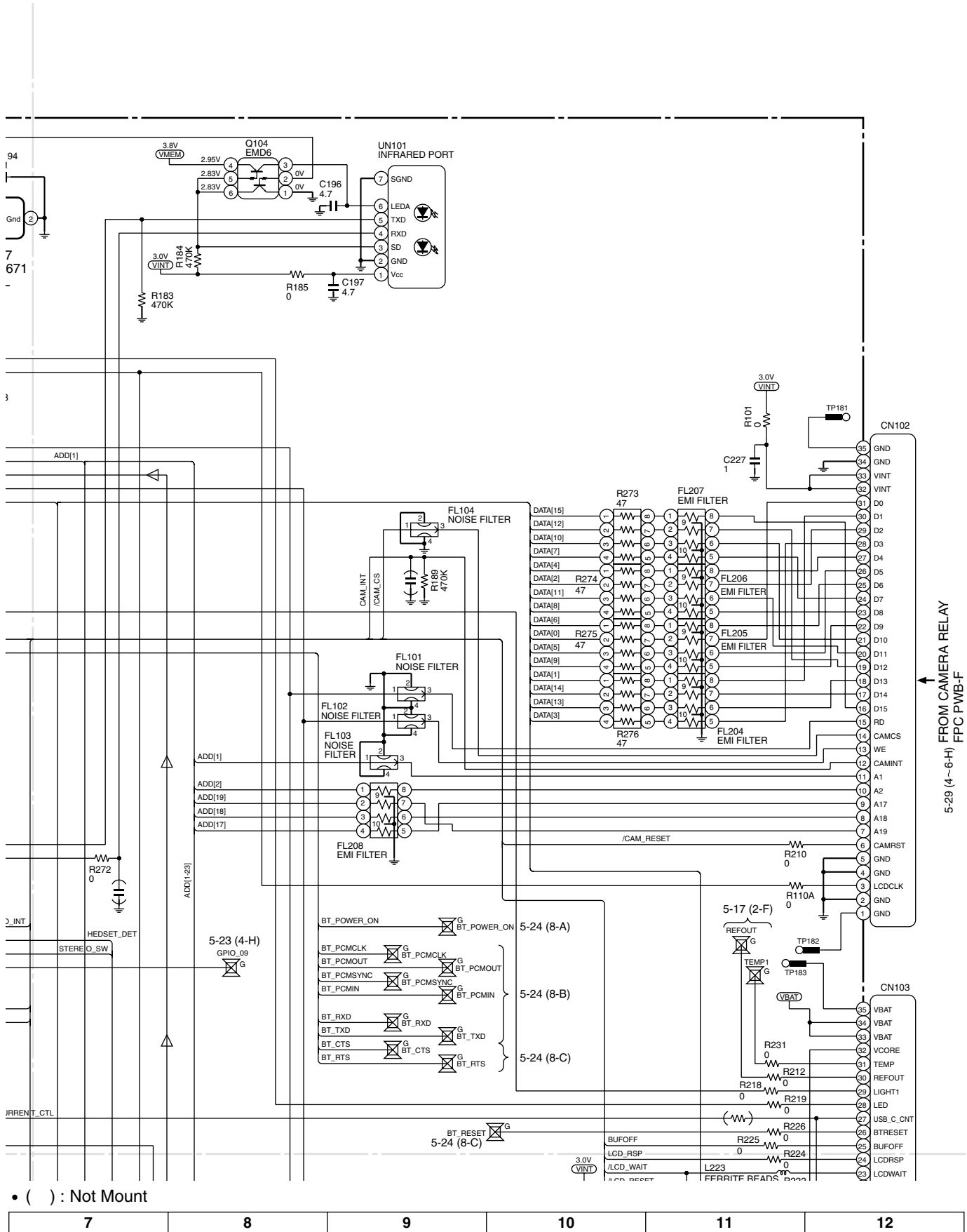
Figure 16 SCHEMATIC DIAGRAM (14/22)
