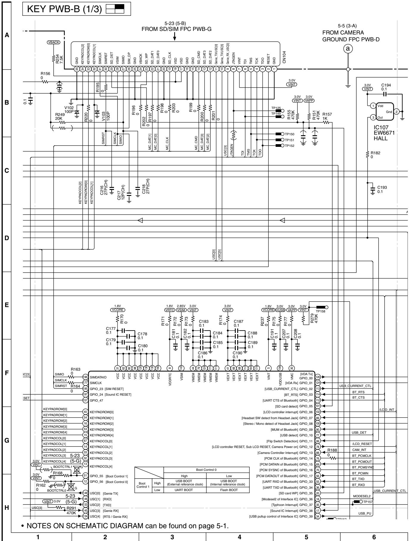
Figure 15 SCHEMATIC DIAGRAM (13/22)
