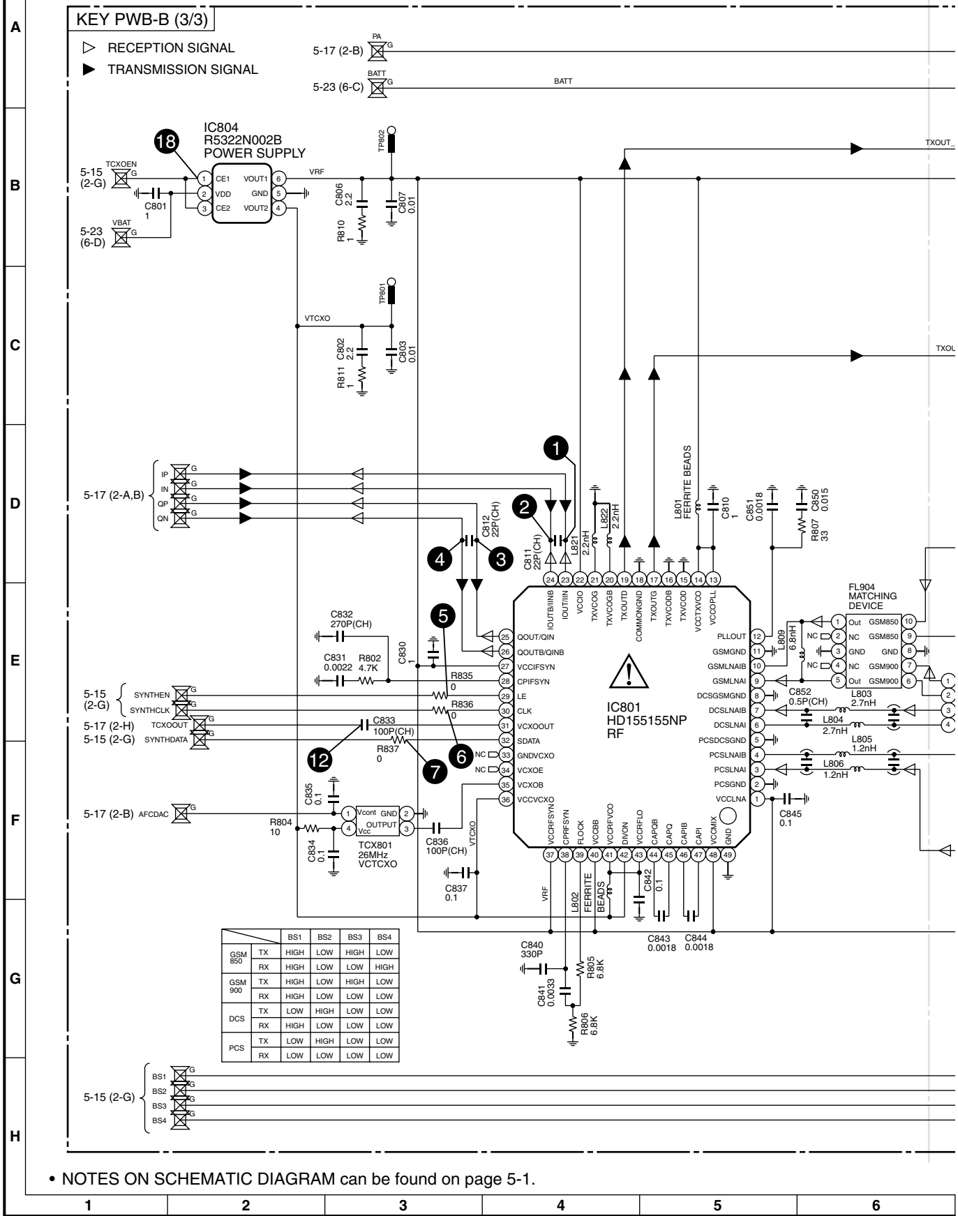
Figure 21 SCHEMATIC DIAGRAM (19/22)
