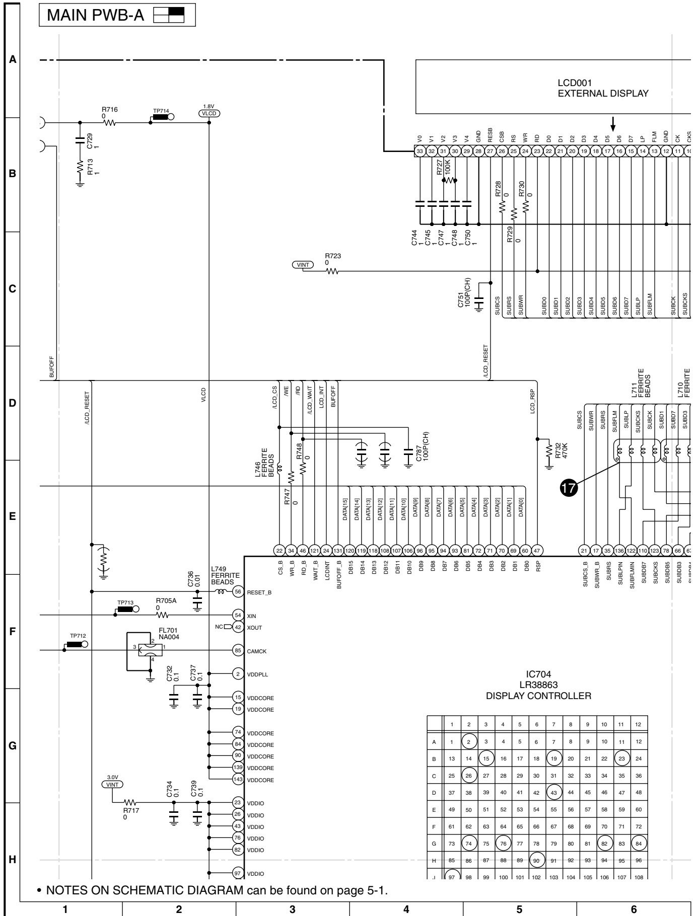
Figure 5 SCHEMATIC DIAGRAM (5/22)
