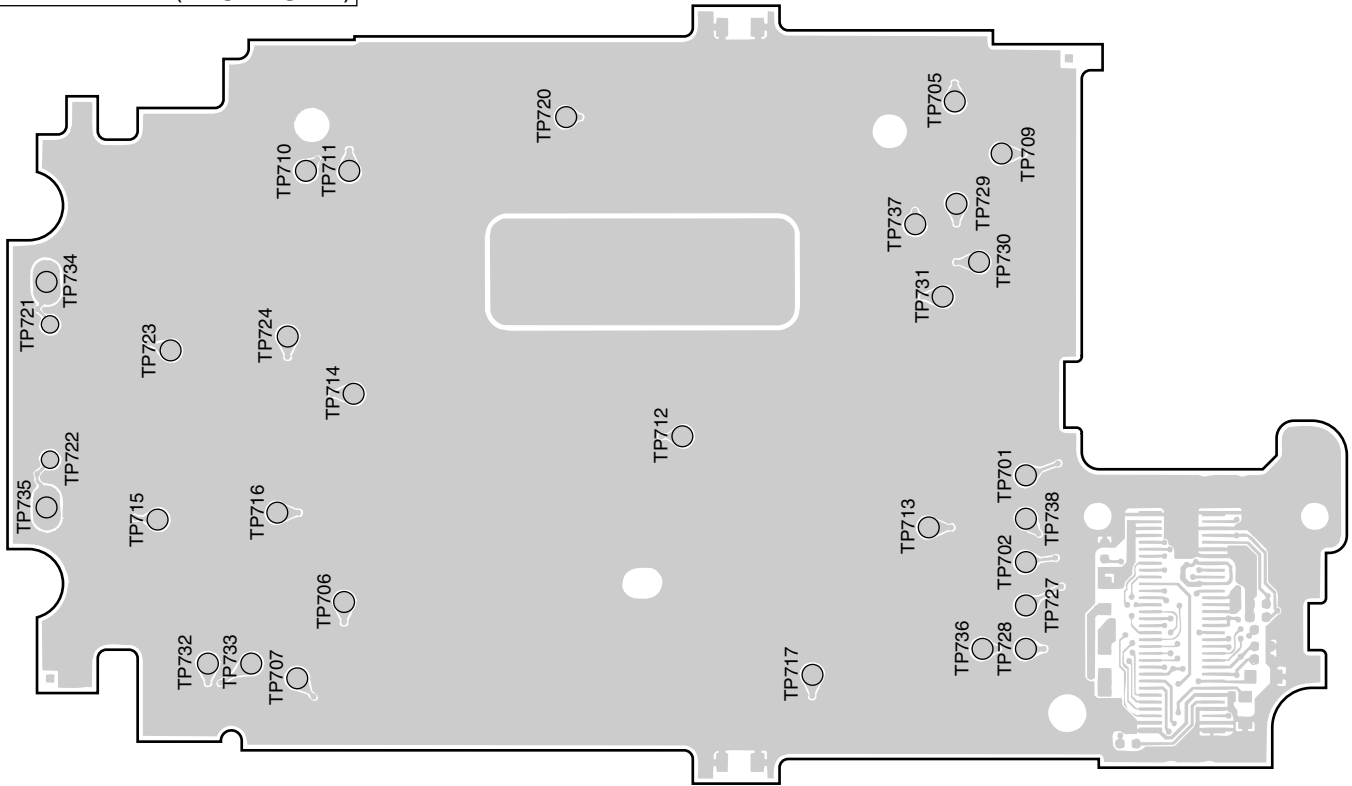
Figure 89 TEST POINT
