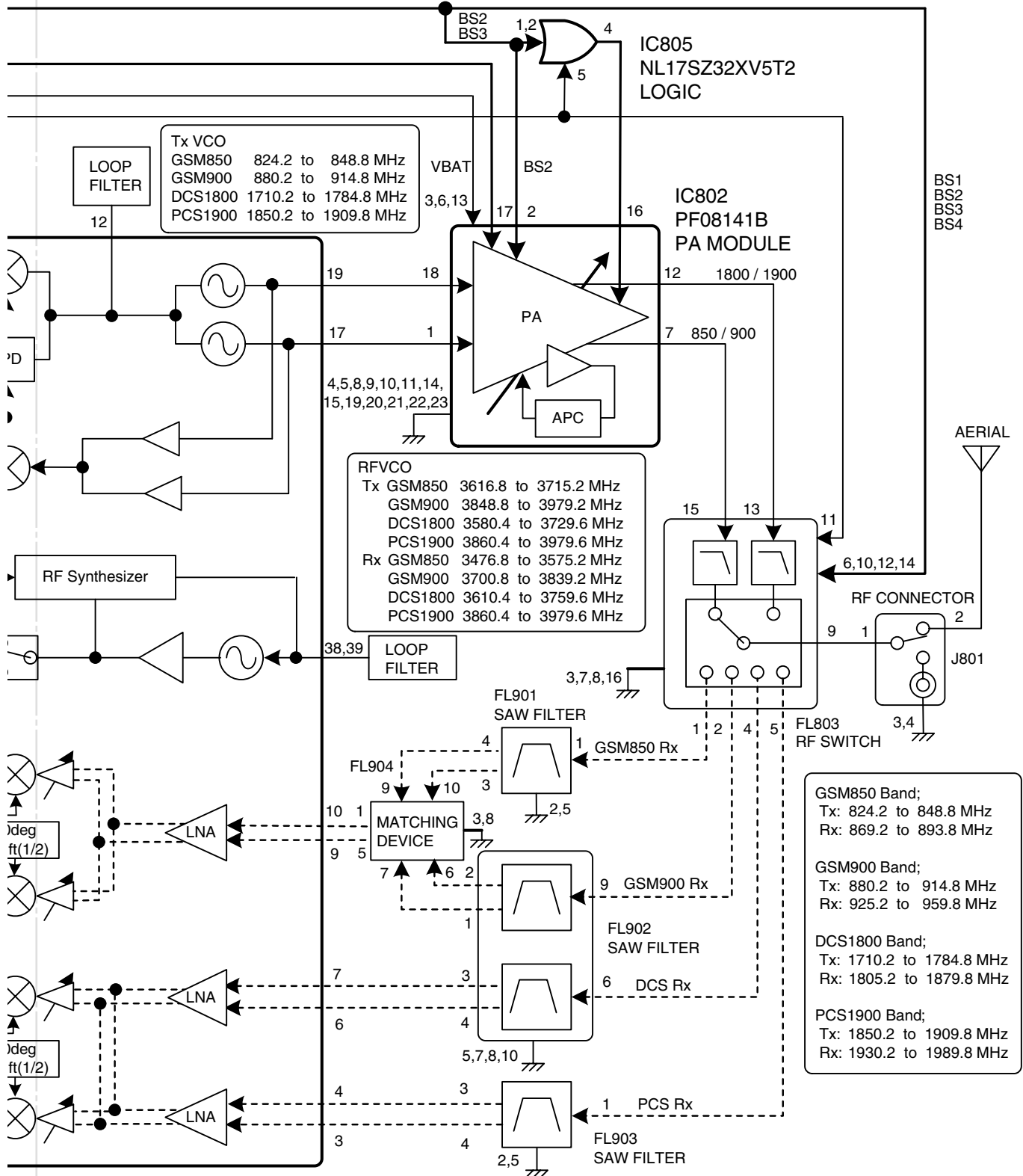
Figure 4 RF BLOCK DIAGRAM (2/2)
