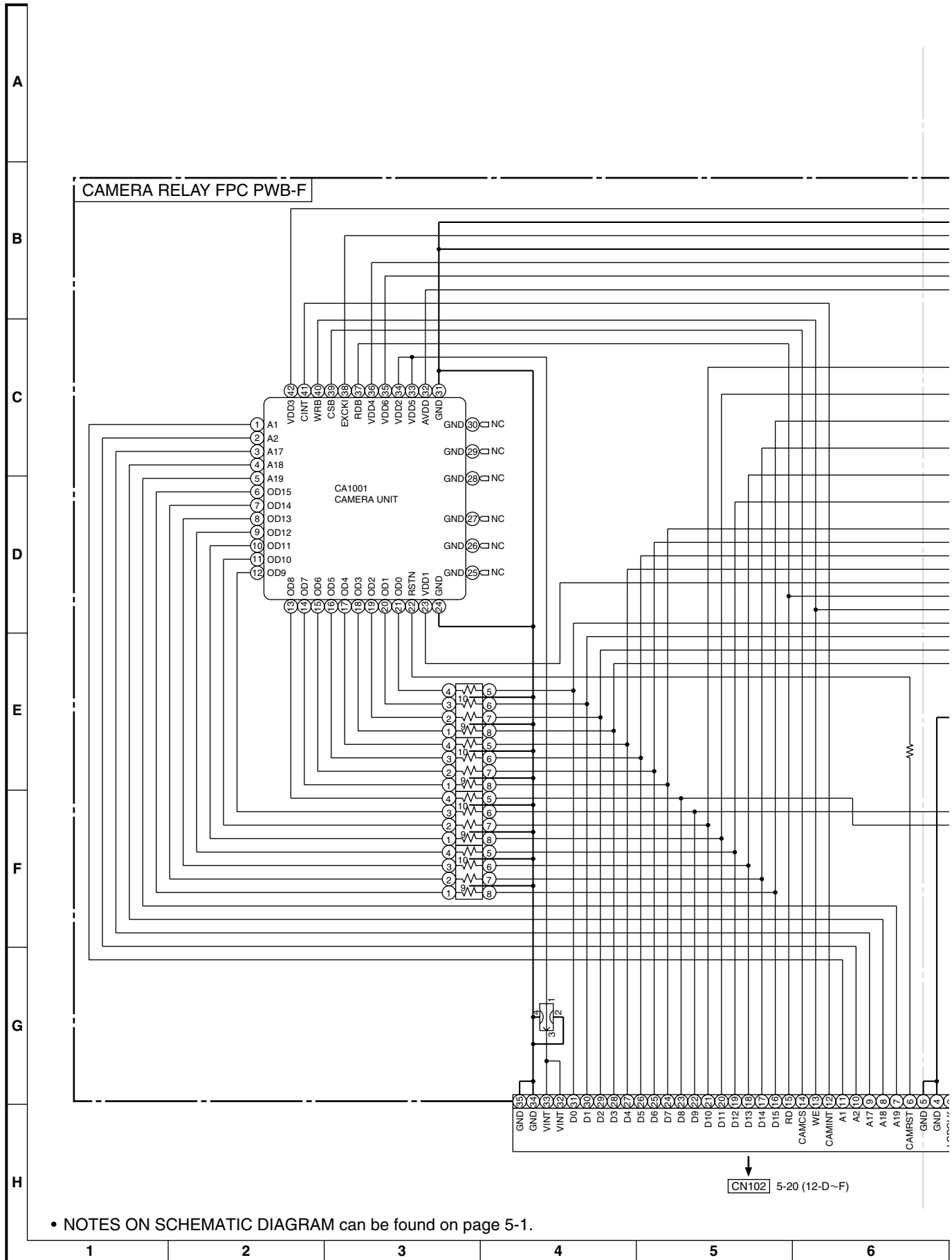
Figure 25 SCHEMATIC DIAGRAM (21/22)
