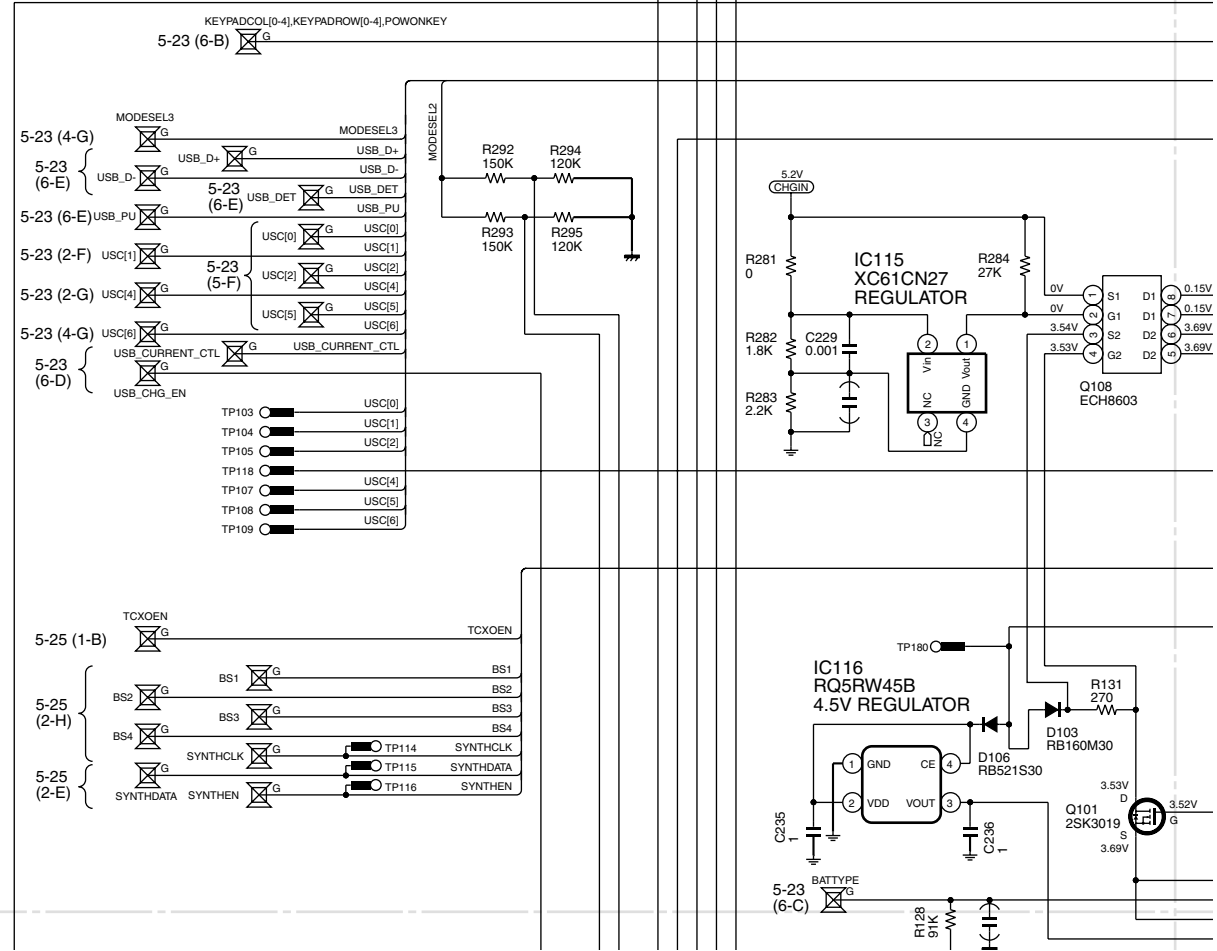
Figure 11 SCHEMATIC DIAGRAM (9/22)
