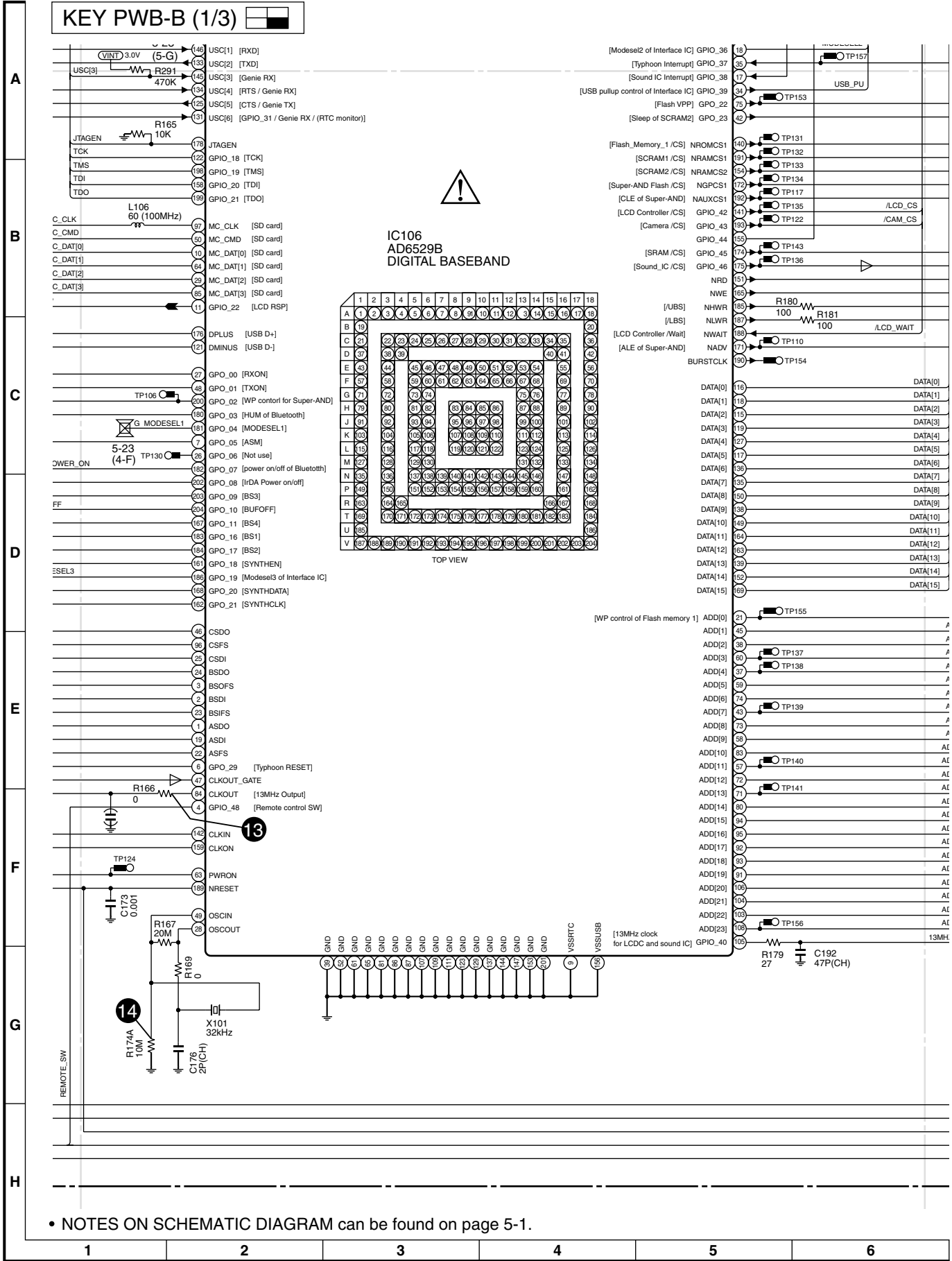
Figure 17 SCHEMATIC DIAGRAM (15/22)
