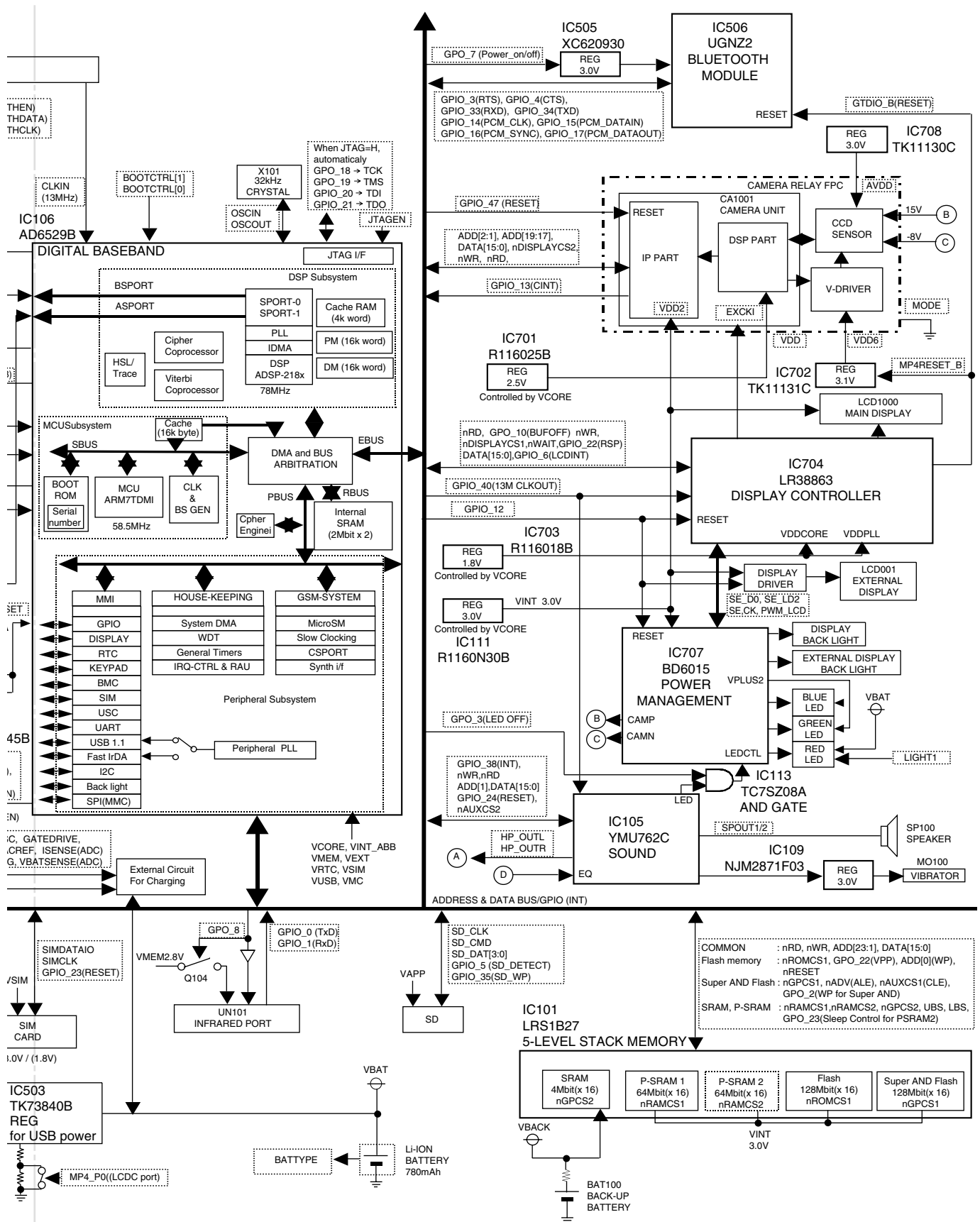
Figure 2 MAIN BLOCK DIAGRAM (2/2)
