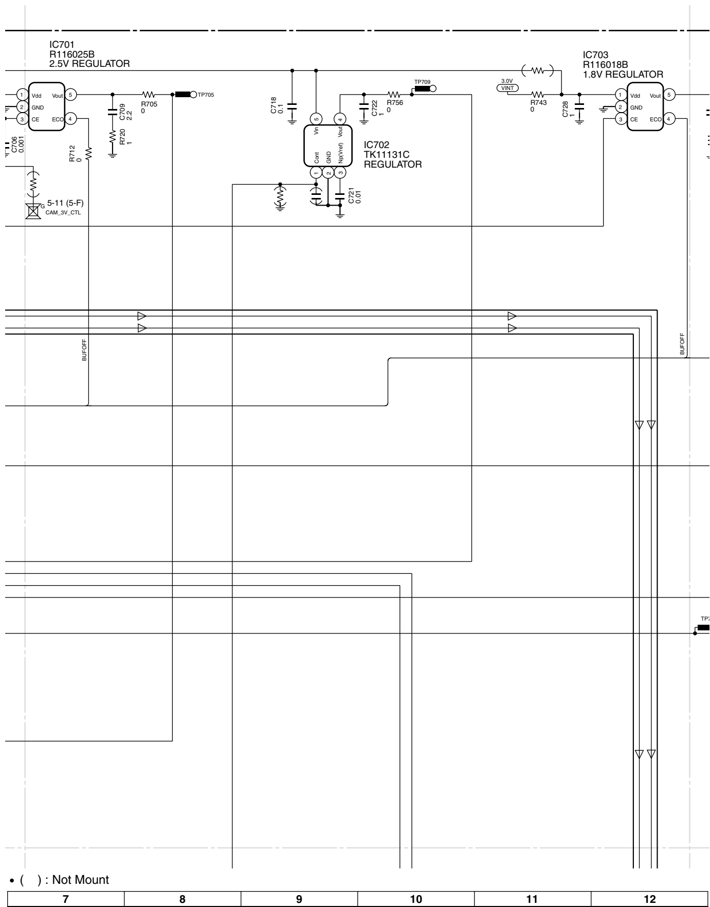
Figure 2 SCHEMATIC DIAGRAM (2/22)
