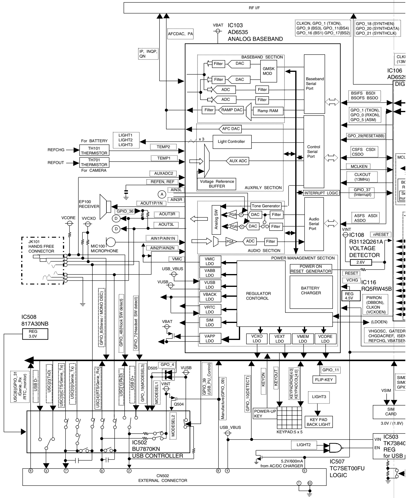
Figure 1 MAIN BLOCK DIAGRAM (1/2)
