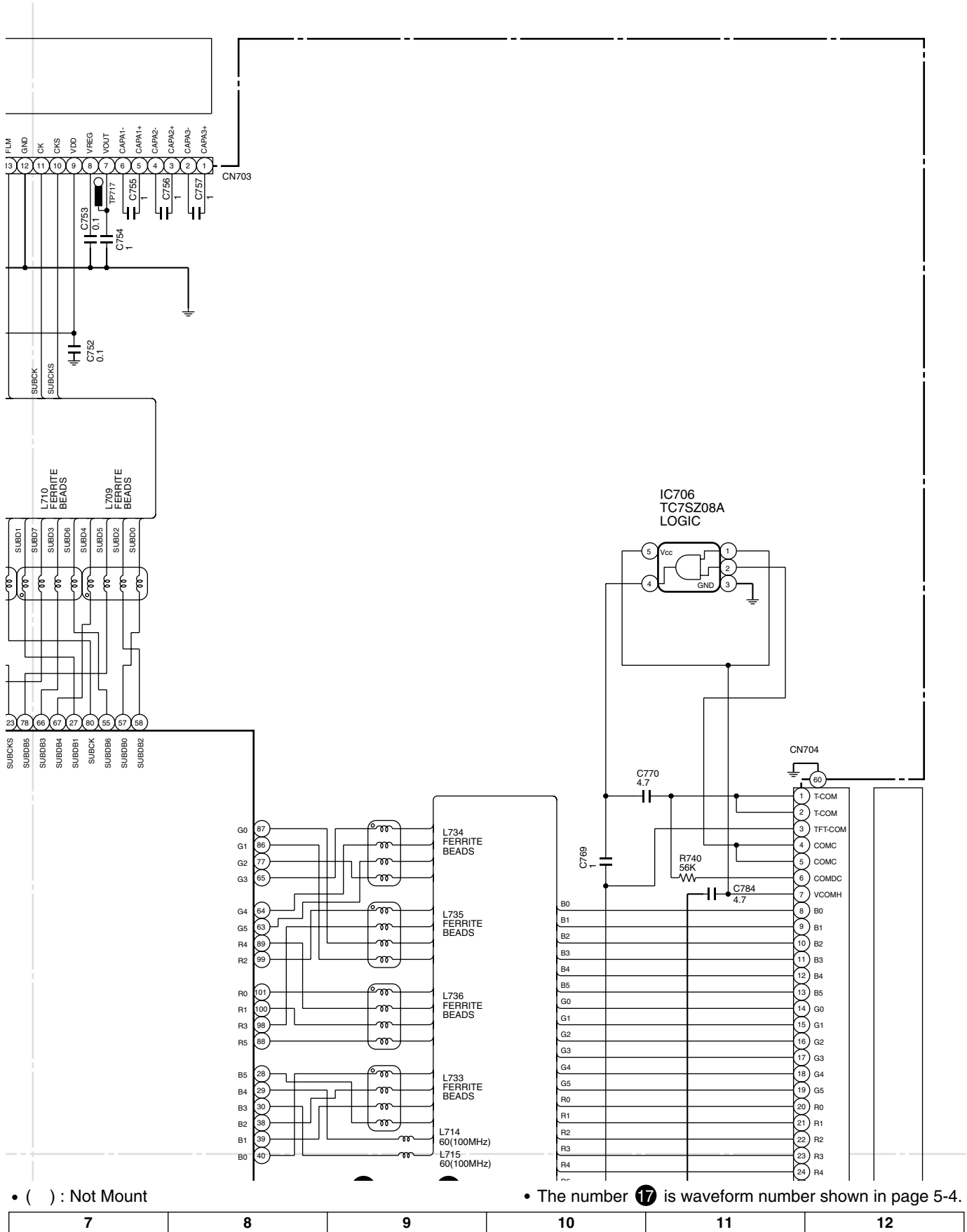
Figure 6 SCHEMATIC DIAGRAM (6/22)
