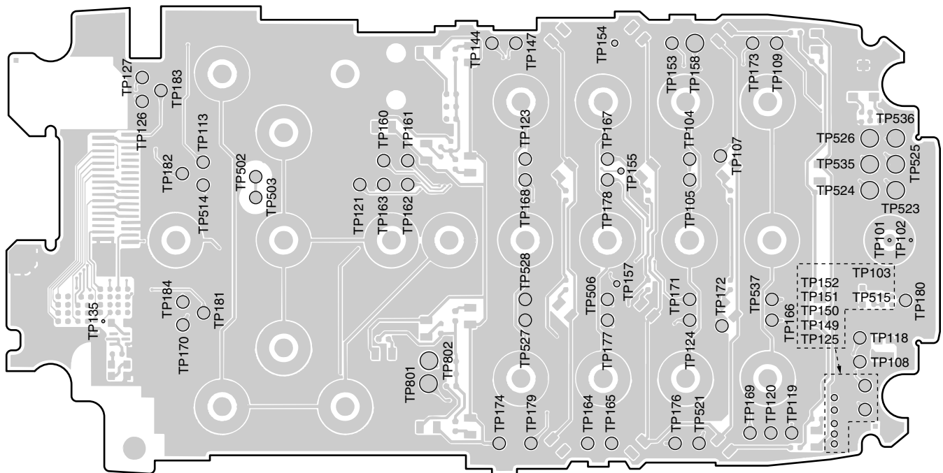
Figure 91 TEST POINT
