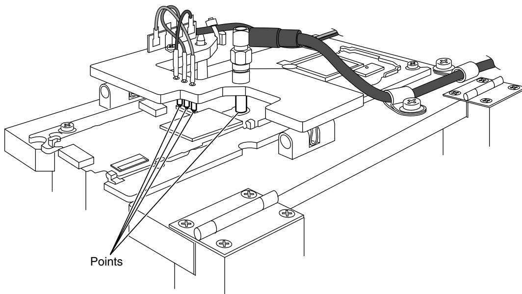
Figure 58 Contact points
