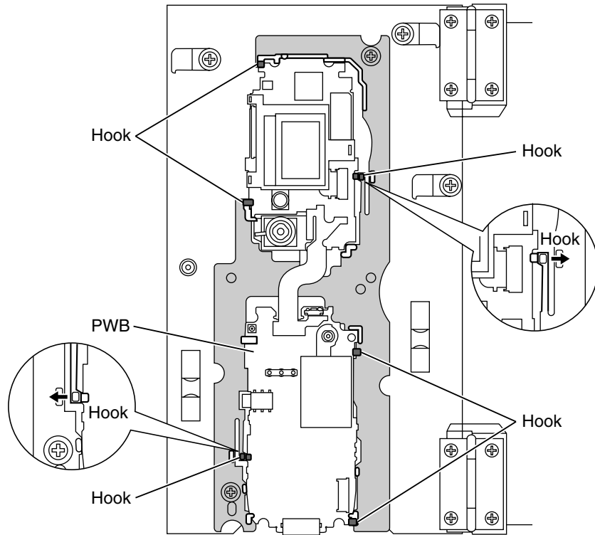
Figure 56 PWB installation
