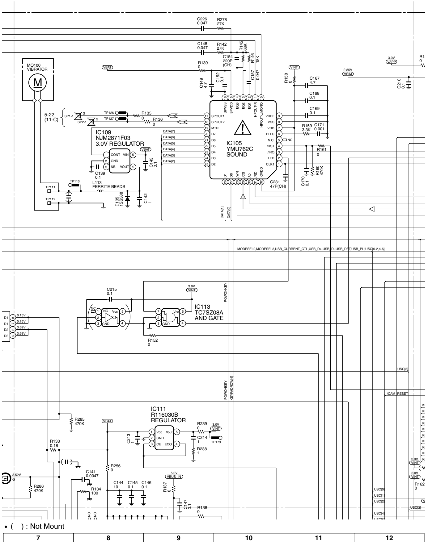
Figure 12 SCHEMATIC DIAGRAM (10/22)
