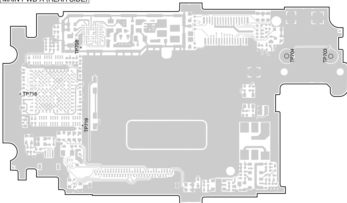
Figure 90 TEST POINT
