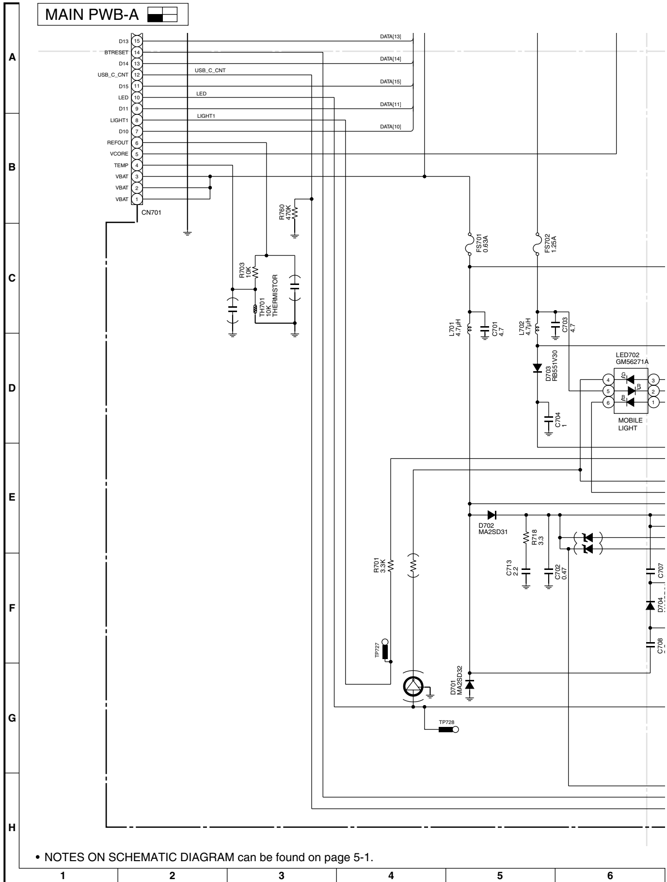
Figure 3 SCHEMATIC DIAGRAM (3/22)
