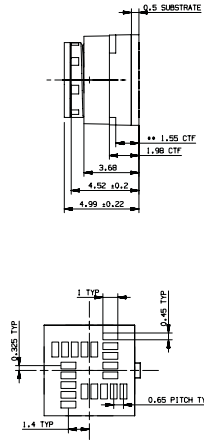
SOCKET CONTACT PADS NICKEL & GOLD PLATED COPPER
