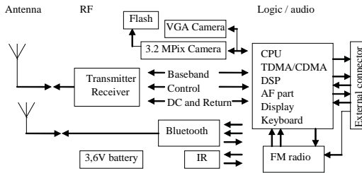
Figure 1. Block diagram of the K800.
