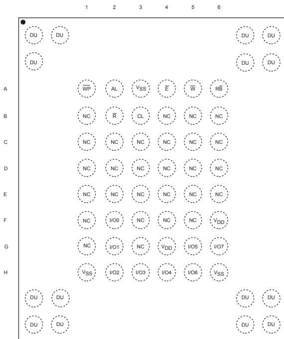
FBGA63 Connections, x8 devices (Top view through package)
