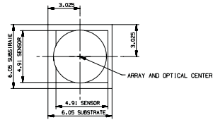
THIS VIEW SHOWS SUBSTRATE AND SENSOR ONLY
