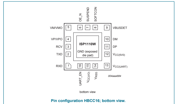
Pin configuration HBCC16; bottom view.
