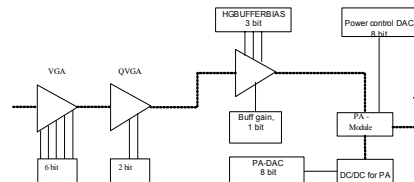
Figure 2. WCDMA transmitter.
