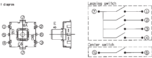
Circuit diagram
