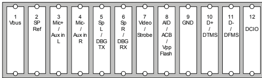
Figure 3. System connector pin out
