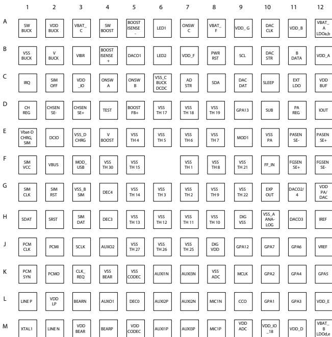
View of Pin Configuration Diagram (as seen from top of package)
