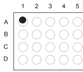
Top View (Bumps down)
