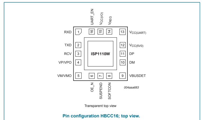
Pin configuration HBCC16; top view.
